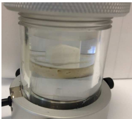
Figure 6: Repair pressure test rig to measure and visualise material response to water
